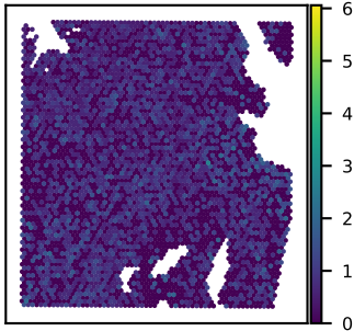
SNU51A LAMA2 expression Moran's I = 0.03
