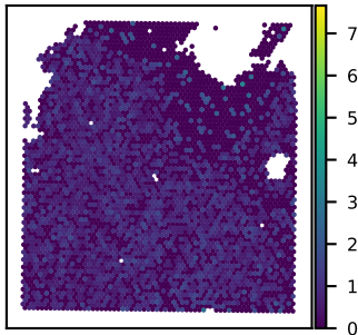
SNU21B CTTNBP2NL expression Moran's I = 0.07
