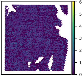
SNU51A TMEM237 expression Moran's I = 0.03
