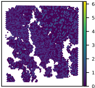
SNU16B SLC39A9 expression Moran's I = 0.01
