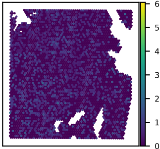
SNU51A TDRP expression Moran's I = 0.02
