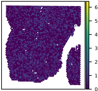
SNU25B KBTBD11 expression Moran's I = 0.01
