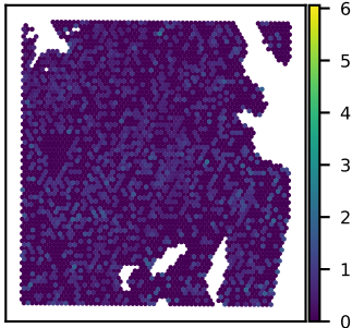
SNU51A SPATA6 expression Moran's I = 0.00
