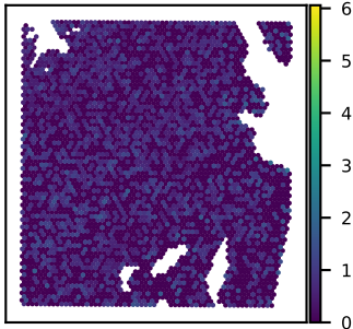
SNU51A KAZN expression Moran's I = 0.01
