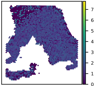
SNU18A CTNND1 expression Moran's I = 0.16
