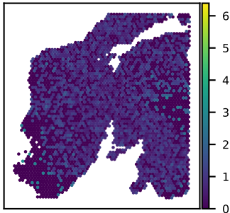
SNU24A ATP5CKMT expression Moran's I = 0.04
