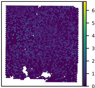
SNU43A SLC10A7 expression Moran's I = 0.03
