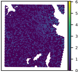
SNU51A GPRASP1 expression Moran's I = 0.09
