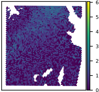
SNU51A DBNDD2 expression Moran's I = 0.26
