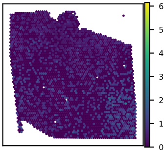
SNU27A CHCHD6 expression Moran's I = 0.04
