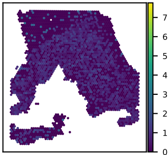
SNU18A C9orf72 expression Moran's I = 0.09
