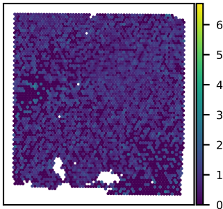
SNU43A TMEM134 expression Moran's I = 0.04
