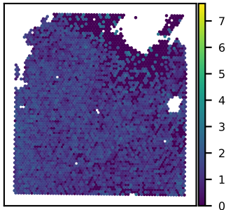
SNU21B TMEM184B expression Moran's I = 0.19
