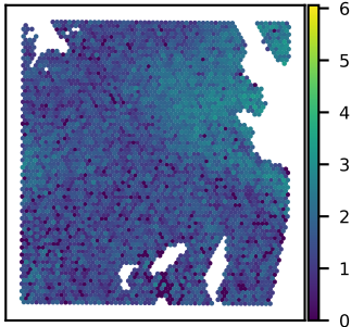
SNU51A TMEM59L expression Moran's I = 0.36
