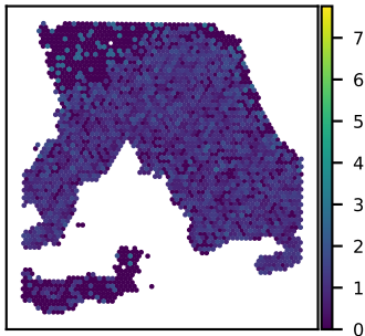
SNU18A C5orf15 expression Moran's I = 0.10
