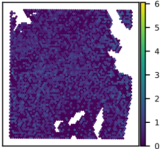
SNU51A KCNA2 expression Moran's I = 0.05
