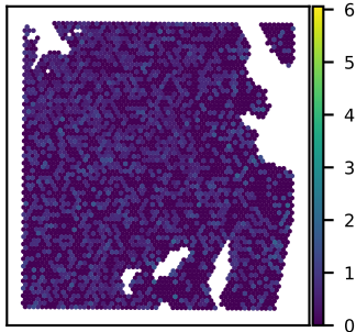
SNU51A NUP98 expression Moran's I = 0.01
