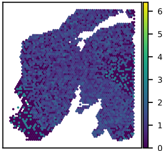
SNU24A SNRNP25 expression Moran's I = 0.03
