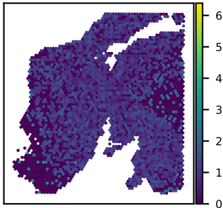
SNU24A CPSF1 expression Moran's I = 0.08
