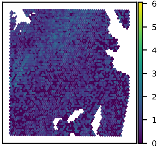
SNU51A C1orf198 expression Moran's I = 0.17
