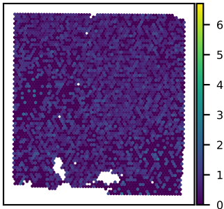
SNU43A NKIRAS2 expression Moran's I = 0.02
