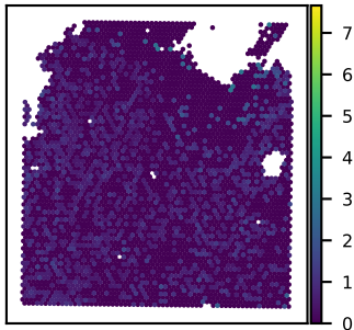
SNU21B STXBP1 expression Moran's I = 0.05
