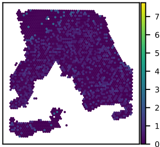
SNU18A ZNF274 expression Moran's I = 0.02
