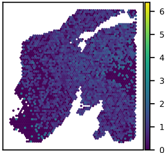
SNU24A TMEM176A expression Moran's I = 0.12
