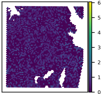
SNU51A LRRC14 expression Moran's I = 0.02
