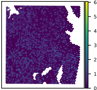
SNU51A SPAG5 expression Moran's I = 0.06
