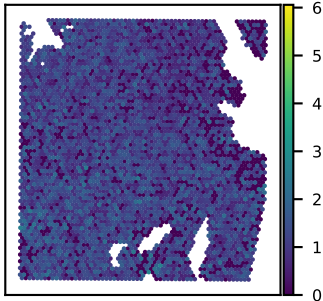
SNU51A IVNS1ABP expression Moran's I = 0.09
