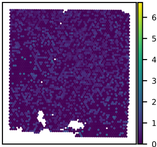
SNU43A C9orf85 expression Moran's I = 0.01
