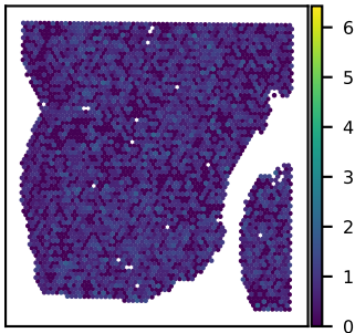
SNU25B LSAMP expression Moran's I = 0.04
