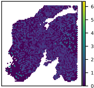
SNU24A RNMT expression Moran's I = 0.03
