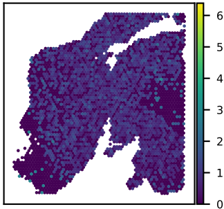
SNU24A SERPINB1 expression Moran's I = 0.10
