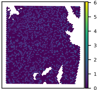
SNU51A ASB8 expression Moran's I = 0.01
