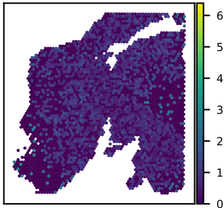
SNU24A RECQL5 expression Moran's I = 0.03
