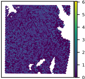
SNU51A PPP2R5A expression Moran's I = 0.04
