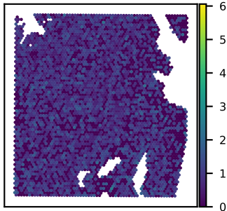
SNU51A OSBPL9 expression Moran's I = 0.03
