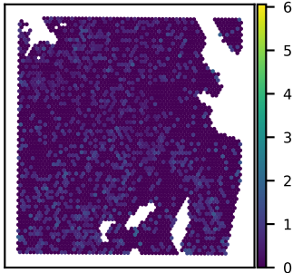
SNU51A EDNRA expression Moran's I = 0.05
