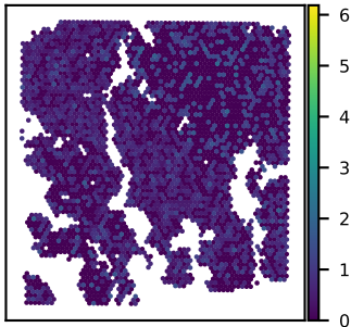
SNU16B SMARCD2 expression Moran's I = 0.02
