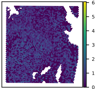
SNU51A LRRN1 expression Moran's I = 0.12
