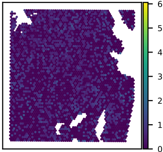
SNU51A TBC1D22A expression Moran's I = 0.01
