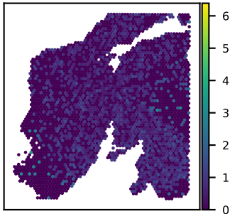
SNU24A B4GALT6 expression Moran's I = 0.06
