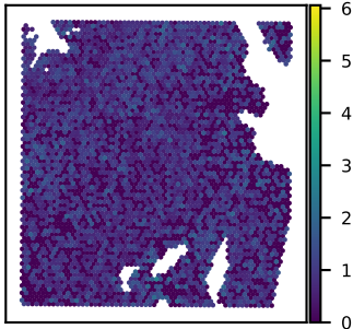
SNU51A MGAT1 expression Moran's I = 0.05
