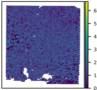
SNU43A COPS6 expression Moran's I = 0.05
