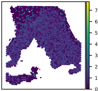
SNU18A KCTD20 expression Moran's I = 0.12
