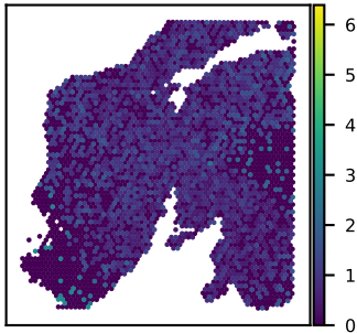
SNU24A GRAMD1B expression Moran's I = 0.05
