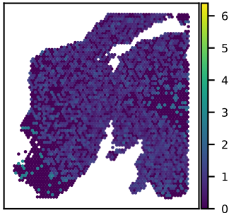
SNU24A EXOSC6 expression Moran's I = 0.06
