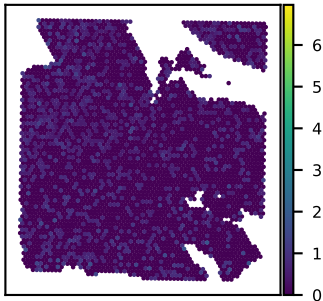
SNU24B PACRG expression Moran's I = 0.02
